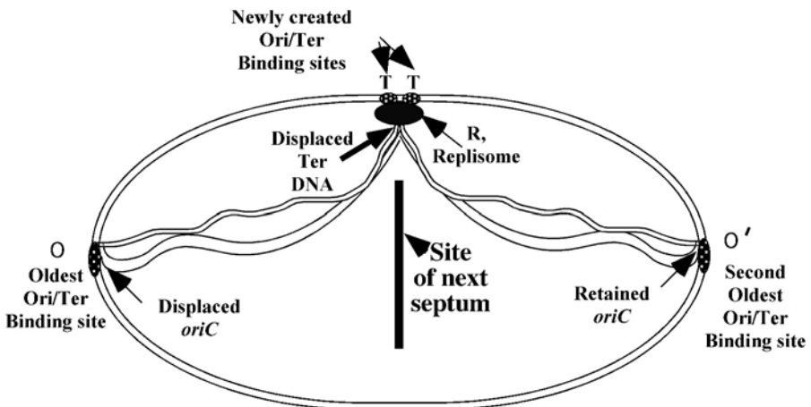
Figure 12.5 Chromosome replication and establishment of next septal location. See text.
