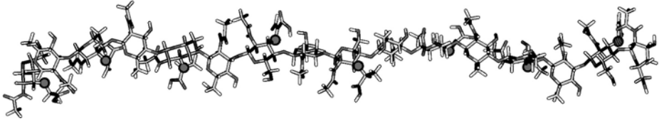
Figure 7.1 The conformation of a glycan of eight polymerized NAM-NAM disaccharides. This chain of 16 hexoses under no external stress forms itself into a helix spontaneously. In this chain, it takes four disaccharides to complete a revolution. This probably defines the conformation of the chains in bacterial walls and hence the two-dimensional structure of a layer of murein. It also leads to the tessera structure of the next chapter. The ether oxygen atoms in the D-lactyl groups of the NAM residues have been enlarged and darkened to make it easy to observe the roughly helical rotation of this relaxed glycan chain.
