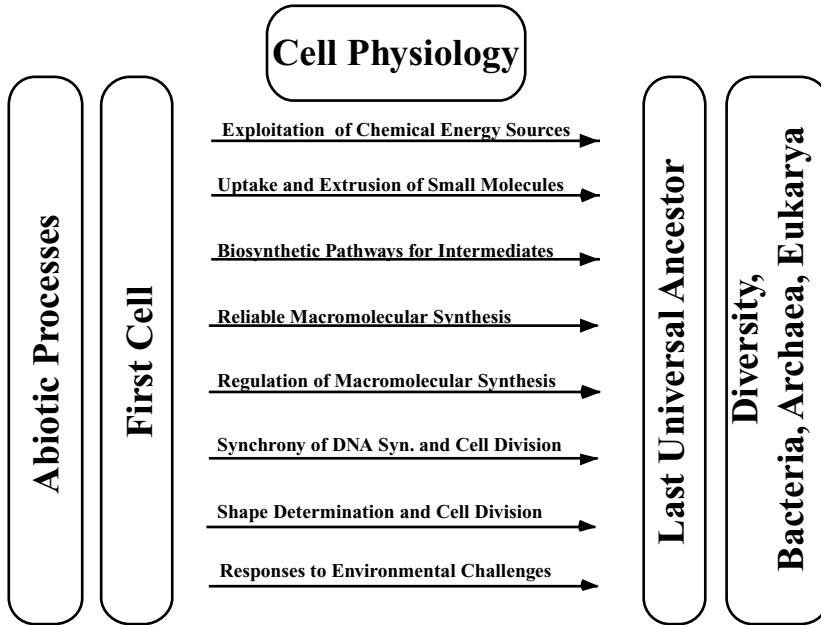
Figure 4.1 The global systems that were perfected before stable diversity developed but after the First Cell arose.
