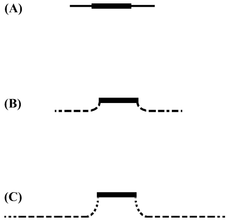
Figure 14.7 The formation of a bulge resulting from an inert patch of sidewall murein. On the top, the thick line segment designates a region that is metabolically inert. As the sidewall grows, as shown in the middle, the inert patch cannot grow, so the patch is moved outward as it is pushed and supported by new growth. This process continues, as shown in the bottom. Other variations on this bulge theme could lead to branches and Y-shaped cells.
