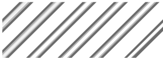
Figure 12.1 Grooves produced by the inside-to-outside growth of Gram-positive rods. As new unstressed layers become added to the murein wall and as they become stressed, they elongate and move outward and form a stress pattern that is not uniform. Where previous grooves have developed and reduced the stress on the surface, there is more stress present at the bottom of the groove than there is where more cleavage takes place. This is a simple case of an analogue of Griffith's law.
