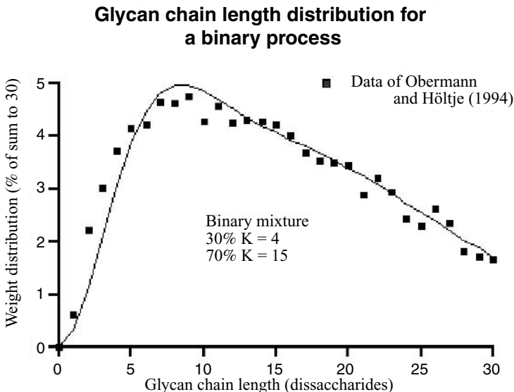
Figure 7.2 The distribution of the glycan chain lengths compared with the experiment. In the fitted distribution two components were assumed.
