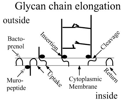
Figure 6.2 Transport, insertion, cleavage, and cross-linking. Shown from the left-hand side is a bactoprenol molecule, then a bactoprenol attached to a disaccharide penta-muropeptide facing the cytoplasm. Further to the right, after transport a bactoprenol attached to a penta-muropeptide disaccharide facing the environment is shown. Still further to the right a pair of growing glycan chains cross-linked at two places is shown. The disaccharide is shown inserted at the base of the chain and the penta-muropeptide is shown unrolled in the environment outside the cell or in the periplasmic space, both of which are hydrophilic. Sites of cleavages for the transglycosylase-mediated insertion step are indicated. The liberated bactoprenol inverts itself through the cytoplasmic membrane to carry another disaccharide penta-muropeptide through the membrane.
