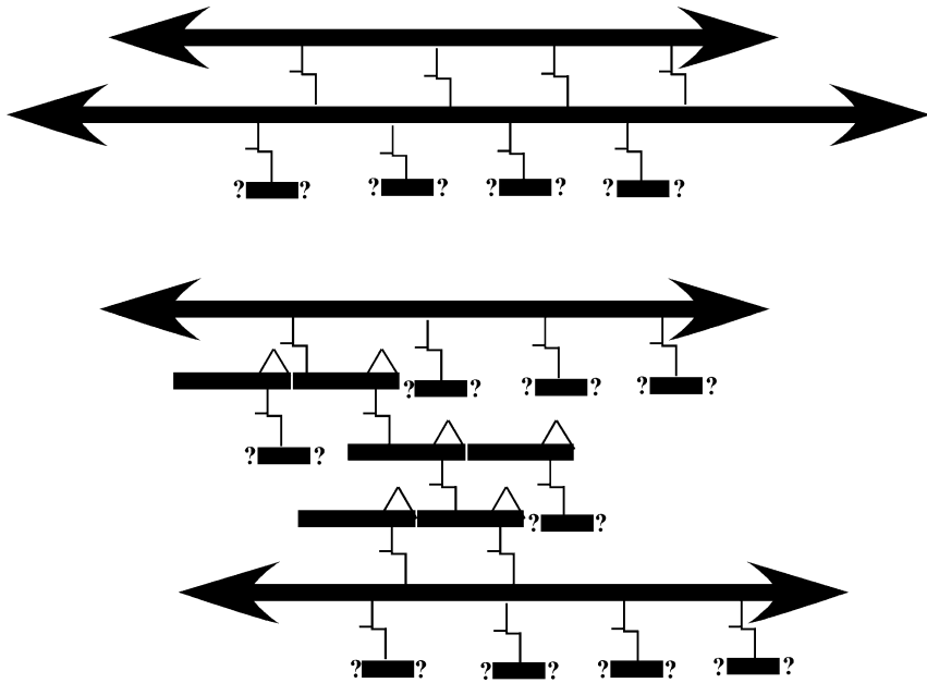
Figure 14.5 Wall architecture of Helicobacter pylori . At the top are shown two glycan chains linked together by octa- or nona-muropeptides. The depiction of the top glycan is inaccurate because each cross-link will point at right angles to that of their immediate neighbors and therefore could not bridge to the next chain. The longer glycan shown connected to it may be bound to other chains or structures like Figure 14.4A or B. The bottom structure shows how structures like 14.4B could function as flexible and longer linkages between glycan such as depicted in Figure 14.4C.
