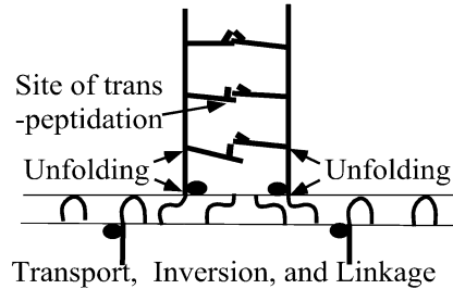
Figure 6.3 Cross-linking. Shown on the bottom, as in Figure 6.2, are the steps of transport, inversion and glycan insertion of the disaccharide penta-muropeptide. The transport of the disaccharide penta-muropeptide unit is shown moved through the phospholipid membrane and inserted into the growing glycan chain. A membrane-bound enzyme, which is a transglycosylase, inserts the growing chains. This results in the new unit's insertion into the nascent wall. The two rolled-up penta-muropeptides unroll and are electrostatically attracted to each other. For the peptide cross-linking, a diaminopimelic acid end of one and the D-ala-D-ala of another peptide chain interact and become attached via the agency of a membrane-bound transpeptidase and with the release of D-alanine. The remaining two ends interact electrostatically to be part of the control system for wall growth.
