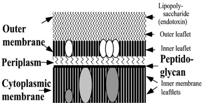
Figure 13.1 The Gram-negative wall in cross-section.
