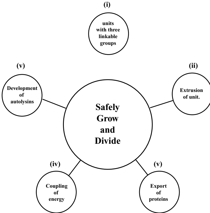
Figure 16.1 Five-component process in murein sacculus formation. The minimum set of processes needed to create an exoskeleton or sacculus includes: (i) metabolic transformations to make disaccharide penta-muropeptides by simple modifications of existing enzymatic steps; (ii) extrusion of the disaccharide penta-muropeptide through the lipid membrane with the help of bactoprenol, also known as unadecaprenol; (iii) extrusion of proteins, such as the penicillin binding proteins (PBPs) and autolysins (the transport of these may have been patterned after secretion of exoenzymes needed for saprophytic growth); (iv) exportable energy in the form of disposable pyrophosphate and the peptide bond in D-Ala-D-Ala to support thermodynamic requirements for building and repairing this structure outside the cell proper; and (v) precise control over autolysins to maintain safe growth.
