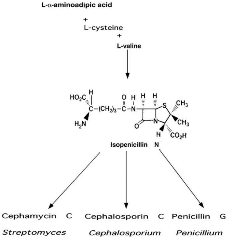
Figure 19.3 Movement of the \beta -lactam pathway from a bacterium into three kinds of fungi. Once the pathway entered into these fungal classes, many minor variations developed.
