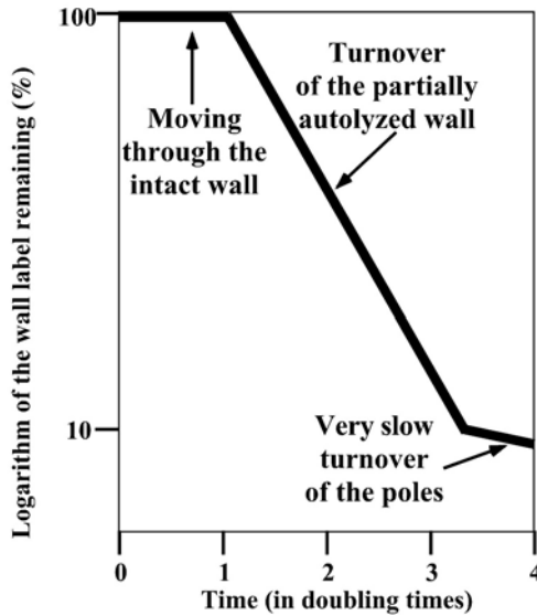
Figure 12.4 Turnover of wall label in a Gram-positive rod-shaped organism. Because of the inside-to-outside manner of cylinder growth, the incorporated label is retained for a generation and then lost exponentially. Finally, only the label in the poles remains.
