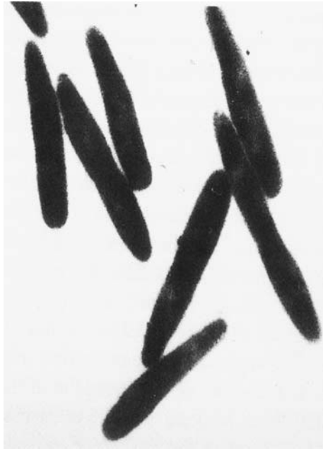
Figure 14.6 Shift-up of E. coli cells from growth in minimal medium into a rich medium. Figure taken from Woldringh et al. (1980).
