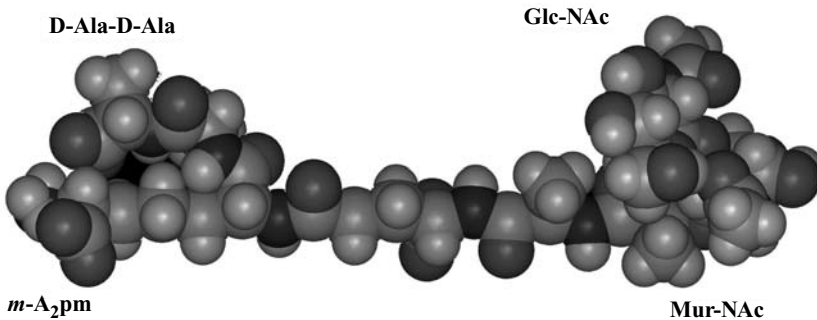
Figure 6.1 The penta-muropeptide of E. coli and B. subtilis . The partially stretched molecular molecule (Koch, 2000) is shown. The right-hand side ends in the disaccharide portion. These sugars allow it to be inserted and to extend the glycan chain. The left-hand side has two ends. One branch ends in a D-Ala-D-Ala-. By transpeptidation it can enter into an amide linkage that is almost identical to an ordinary peptide linkage. The other branch ends in a zwitter ion, which is composed of a carboxyl and an amino group. The amino group from one penta-muropeptide may interact with the penultimate D-Alanine from another penta-muropeptide to form a tail-to-tail bond to cross-link the murein. The central region consists of amino acids in peptide linkage. Some of these amino acids are special because they are D instead of L. One amino acid is glutamic acid linked at its \gamma position instead of the usual \alpha linkage.
