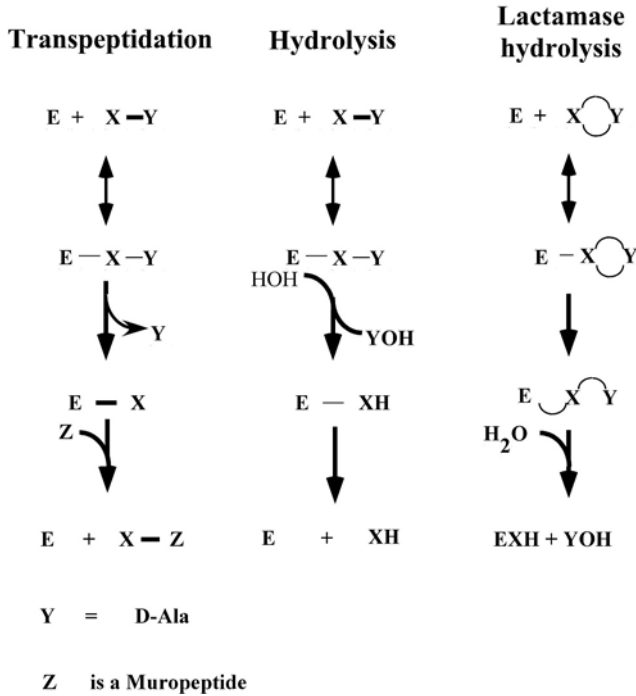
Figure 19.5 Enzymatic pathways of three types of enzymes that deal with a chemical bond that may be called in particular circumstances an amide, a peptide, or a lactam. However, these are different and lead to different outcomes.
