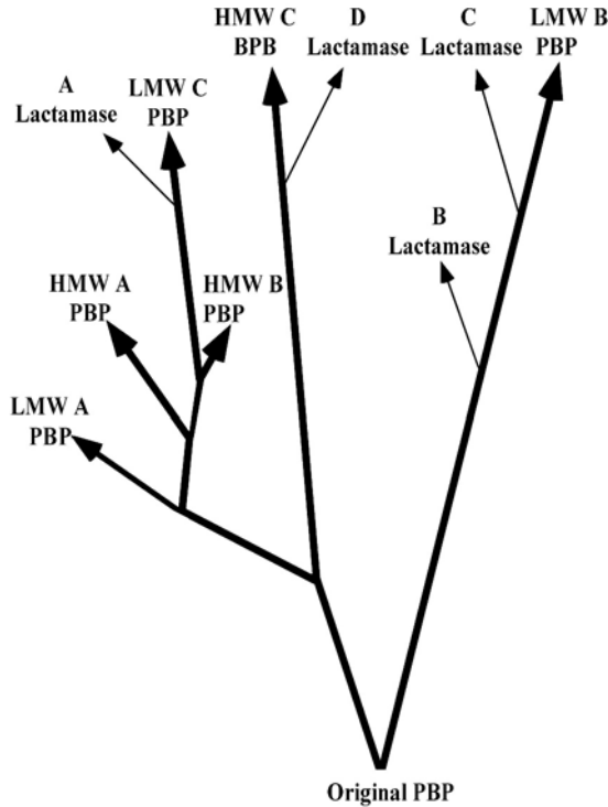
Figure 19.4 The evolutionary tree of penicillin binding proteins (PBPs) and \beta -lactamases. Taken from Koch (2000).
