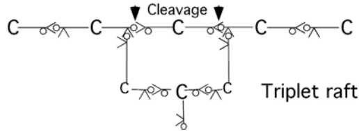
Figure 11.4 The three-for-one model of Höltje. The model proposes that a number of enzymes function together as a holoenzyme to simultaneously both attach new murein to the wall and to cleave the wall in such a fashion that the new material is pulled into the stress-bearing wall to enlarge it (Höltje, 1993). A key point to the model is that a chain of three penta-muropeptides wide and as long as the template strand on a stress-bearing glycan chain are bound to each other and this triplet raft is bound to the template glycan strand in the stress-bearing wall and, as shown, to enclose this glycan chain that is then cleaved out, replacing one chain with three of the same length.
