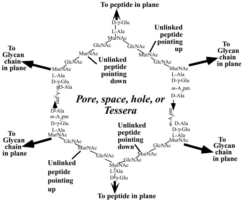
Figure 8.2 The Tessera. This view is more detailed than Figure 8.1, but both emphasize that the tessera is the framing around the pore that the cell uses for transport materials into and out of the cell. Notice that a different set of abbreviations is used than was used above with MurNAc for NAM and GlcNAc for NAG.
