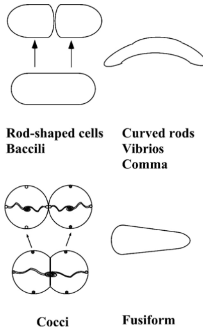
Figure 14.1 The range of shapes of the major types of bacterial cells. This collection idealizes the four types of basic morphology. The rod and the coccus are shown in the division part of their cycles. The curved rods can vary in the degree of their curvature and the fusiform organisms can vary in their taper. Cells with bulges and irregular shape are not shown here.
