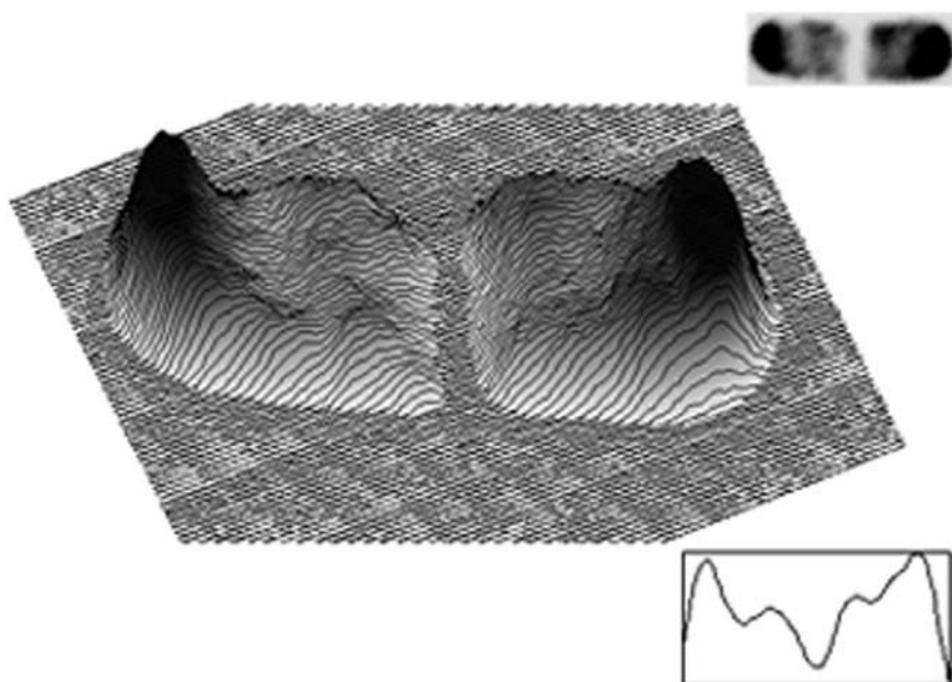
Figure 11.2 Several views of the age distribution of a cell chased for one doubling. The large image is equivalent to the model shown in Figure 11.1 in that it has a cylindrical region of the two cells produced by division. The upper right directly shows the fluorescent image and the lower right image shows the fluorescent density of a longitudinal section.
