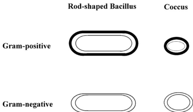
Figure 16.2 Four types of bacteria, one of which might have been the first bacterium. This first bacterium could have had the thick wall of Gram-positive or the thin wall of Gram-negative cells. It could have been rod-shaped or an almost spherical coccus. The text discusses the possibilities of each of the four being the first member of the Bacteria. Note that a variety of more complicated shapes are not included, nor are various kinds of appendages, pili, fimbriae, and flagella, considered at this point.
