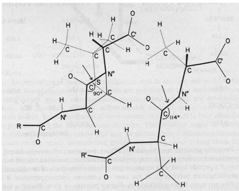
Figure 19.1 The structural stereo-formulae for acyl-D-alanyl-D-alanine (lower) and penicillin (upper). Figure taken from Waxman and Strominger (1982). The similarity between these two structures was the first evidence that \beta -lactam molecules can enter the active site in the transpeptidase and bind to it. Because of the bond stress in the 4-membered ring, it can covalently react and inactivate the enzyme, resulting in blocked sacculus growth and lysis. The arrows indicate the lactam bonds, which are similar to peptide or amide bonds.
