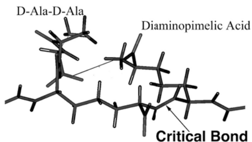
Figure 19.6 The critical bond formed by the endopeptidase PBPs that are the target of \beta -lactams. This linkage is marked with an arrow). Also shown is the relationship of the amino group of the diaminopimelic acid and the carboxyl group of the D-Alanine. This charge interaction occludes entry to the critical linkage area until stress is applied to the non-muropeptide.
