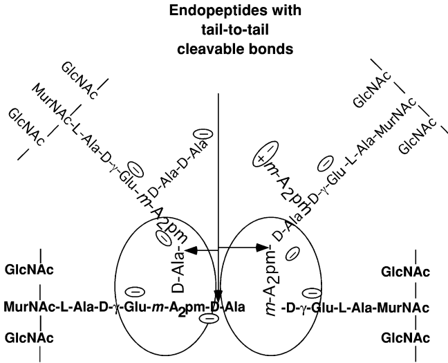
Figure 7.4 The Nona-muropeptide model for wall growth in Gram-negative bacteria. A Nona-muropeptide is shown at the bottom. Above it have been attached two penta-muropeptides. The ellipses represent the transpeptidase molecules that have linked them. A third arrow indicates where an autolysin can enter and cleave the old tail-to-tail bond that must be split to allow enlargement of the wall
