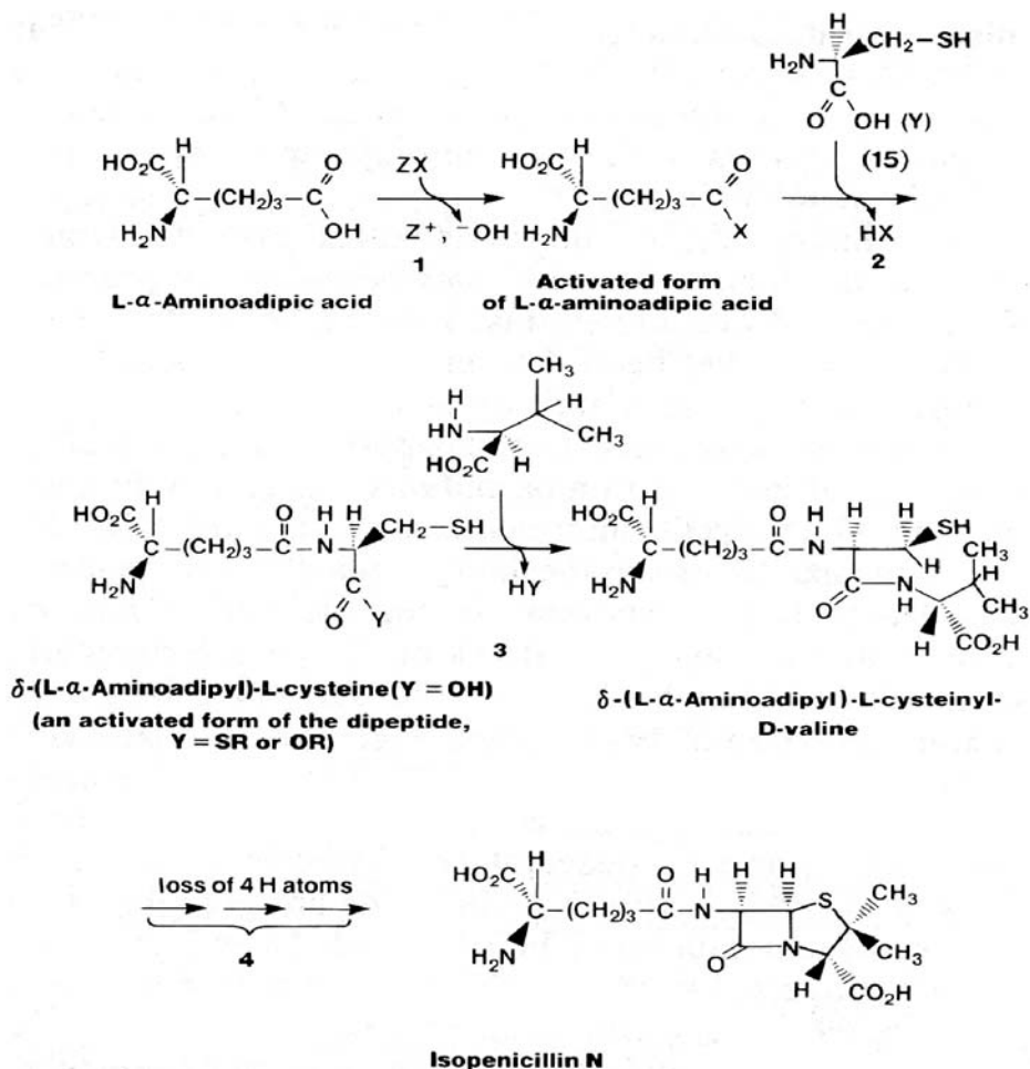
Figure 19.2 Biosynthesis of iso-penicillin N. Taken from Queener and Neuss (1982).
