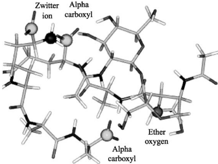
Figure 9.1 A murein unit in the conformation suitable for transport through the membrane. A computer simulation (Koch, 2000) is shown of a penta-muropeptide in an environment simulating the hydrophobic environment of the cytoplasmic membrane. The important point about this structure is that the adopted conformation brings the zwitter ionic group at the end of the diaminopimelic acid to be positioned closely to the \alpha -carboxyl group of the D-glutamic acid of the penta-muropeptide chain. Energy minimization led to a conformation with the amino group located between the two-carboxyl groups and thus the hydrophilic character of these ions is partially lost. This would help the penta-muropeptide to expose a more hydrophobic exterior as it is passed through the phospholipid membrane. In this figure the charged groups are emphasized and marked by the balls on the carbon atoms attached to the groups that have net charges. In addition a ball is located on the one oxygen atom that is in ether linkage. This atom connects the disaccharide to the penta-muropeptide chain in the wall unit.
