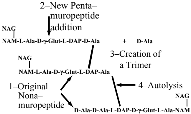
Figure 7.5 The generic model for wall enlargement. The steps in the enlargement start with: (1) a nona-muropeptide within the wall. It had been formed from two penta-muropeptides previously. (2) A new penta-muropeptide enters and is bonded by transpeptidation to a free group of the nona-muropeptide. The D-Ala that is liberated escapes. (3) The transpeptidation forms the trimer, which is composed of three muropeptides. The trimer is decomposed in the fourth step by an autolysin to complete the enlargement by the safe incorporation of a penta-muropeptide.
