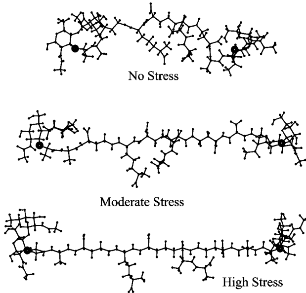
Figure 7.3 Nona-muropeptide at three degrees of stress. The conformation in an aqueous environment of a nona-muropeptide under various degrees of elongation is shown. The conformations from top to bottom are of low, intermediate, and high stress.
