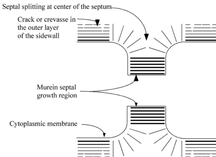
Figure 10.1 A potential explanation for the metabolic inertness of the Gram-positive septum and pole. The inside-to-outside growth mechanism for the sidewalls, discussed in more detail in Chapter 12, is diagrammed. The wall is laid down in layers. Subsequent layers push the earlier ones outward and they become elongated as the cell grows. Eventually they cannot stretch any more and are then split and discarded by an autolytic process.
