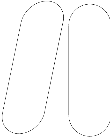
Figure 14.2 Two idealized experiments with a soap bubble pipe. See Figure 11.1 for a photograph of a soap bubble blown between two ridged ends, this process can produce a soap bubble in a cylindrical shape. On the left side of this figure, I show an idealized rod-shaped cylindrical bubble generated as shown in Fig. 11.1. This is formed if the two ends are rigid. It will be cylindrical if the amount of air blown in the bubble is such that the cross sectional area of the bubble is equal to the area of the rigid poles. This construction is feasible, if these rigid plastic ends have been wetted with the soap solution. Then they will not break the bubble when it contacts these solid surfaces. Although not shown in the Fig. 11.1, but one of the rigid ends has to be connected to a tube through which air can be introduced so that a cylindrical bubble can be formed. The amount of air to be introduced would depend on the area of the rigid endplates and the length of the cylinder. The additional issue, relevant to this chapter, is that even if the endplates are not co-linear (as shown on the right-hand side) a right-cylindrical bubble is still produced and is not curved.
