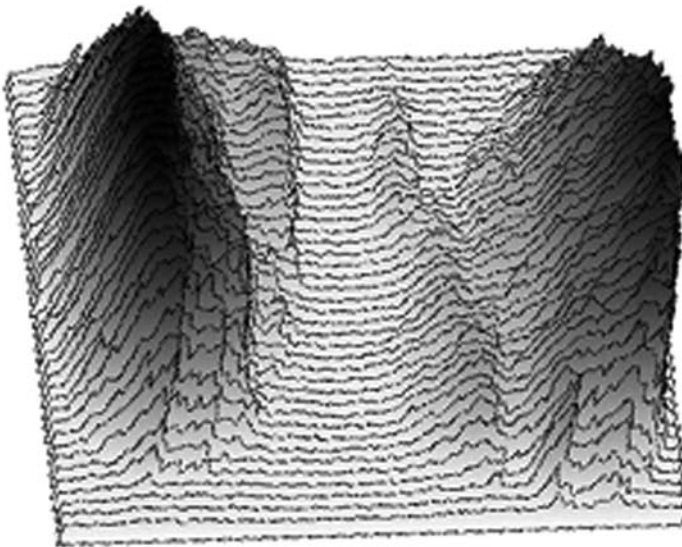
Figure 10.3 A different representation of a cell dividing after one generation of chase. The representation of the older murein present in the sacculus is at a higher elevation in the figure. It can also be seen that the photographic saturation process itself decreased the amount of old murein at the poles. If this had not occurred the elevation would be higher than shown.
