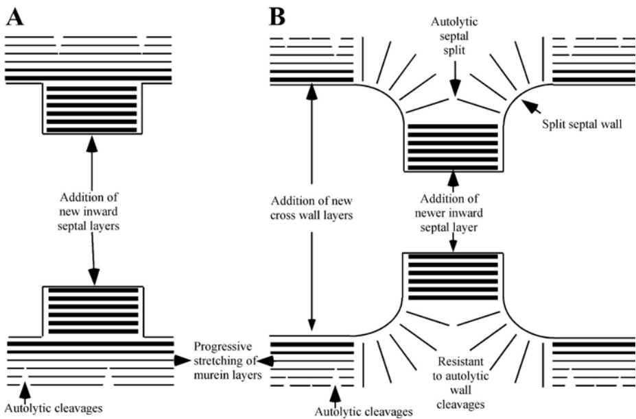
Figure 12.2 Bacillus subtilis septal and pole growth pattern. Panel A shows where new layers are laid down to form a septum. It also shows autolytic cleavages in the outermost wall. Panel B shows the autolytic split that bisects the septum while it is still being completed. Only after the split occurs does the wall stretch to yield a pole in which the layers are perpendicular to the surface and not parallel to it as in the sidewall. This yields, it is postulated, a resistant pole that because of the murein orientation is not subject to the action of autolysins as would occur in the sidewall.
