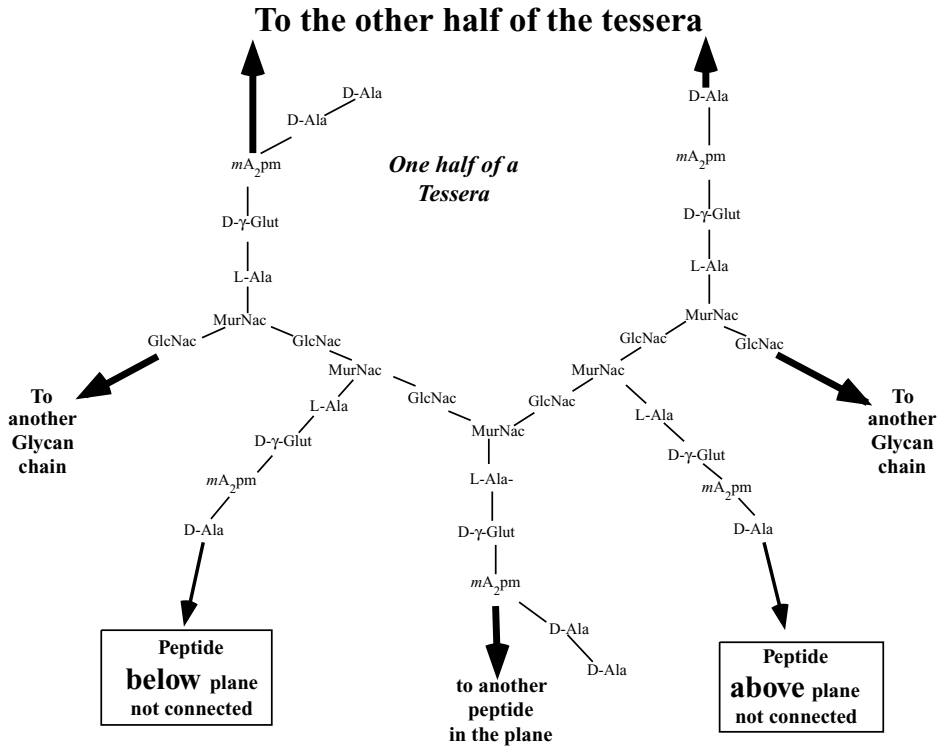
Figure 13.2 One half of a tessera. A tessera in a functional wall is linked to six other tesserae. This takes place via the bold arrows, only half of which are shown. In addition there are mucopeptides extending upward and downward, shown by thinner arrows. In a Gram-negative organism with very thin walls, these are not attached to murein and may be degraded from the forms shown here.
