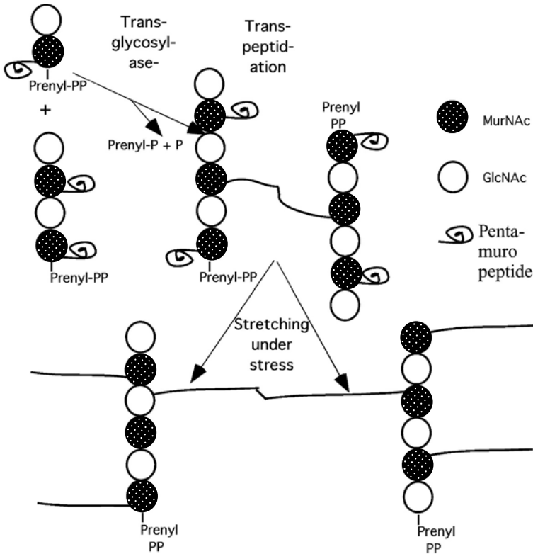
Figure 9.2 Wall formation. The diagram shows the wall growing process as viewed from above the cytoplasmic membrane. On the upper left, the bactoprenol-linked disaccharide penta-muropeptide is shown being attached to the terminal region of a growing chain. Hydrolysis of the pyrophosphate linkage supplies the energy for the formation of the glycosyl bond and drives it to completion. The prenyl-P turns around to face the other side of the membrane in order to engage in forming another disaccharide penta-muropeptide. The liberated phosphate is pumped into the cell. The growing chains form endopeptide bonds as shown on the upper right side. At this point the nona-muropeptide is in a relaxed conformation, but as the cell grows the murein is stretched and stressed.
