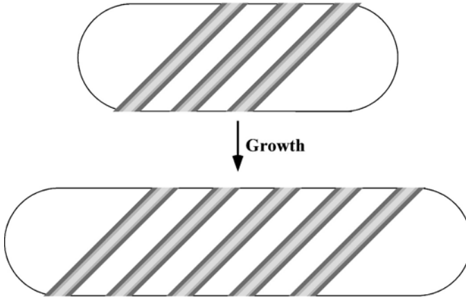
Figure 12.3 Growth with propagation of helices. This figure diagrams the elongation of a helical grooved cell. This leads to growth of the helical grooves of a constant angle with respect to the cell body.
