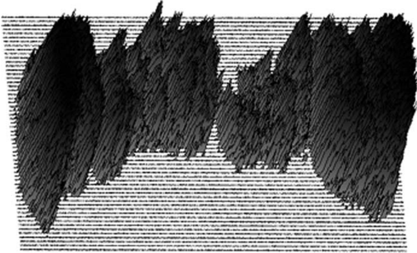
Figure 11.3 Evidence that the age of wall sections varies throughout the cell and that the pole regions are the oldest. This is a two-generation chase of a D-Cysteine labeled bacterium in the presence of aztreonam to block cell division. This figure shows that the sidewall after this length of chase is composed of largely old segments interspersed with new wall. Although it appears that this fluorescent micrograph is two cells and not one, other representations showed that the entire body of this cell is only one cell.
